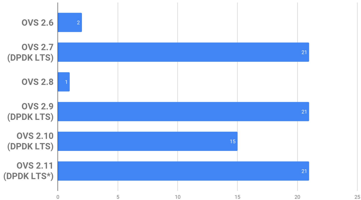
Months of DPDK support after OVS release
